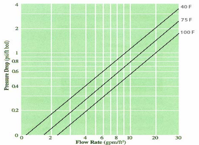
Pressure Loss Curve
