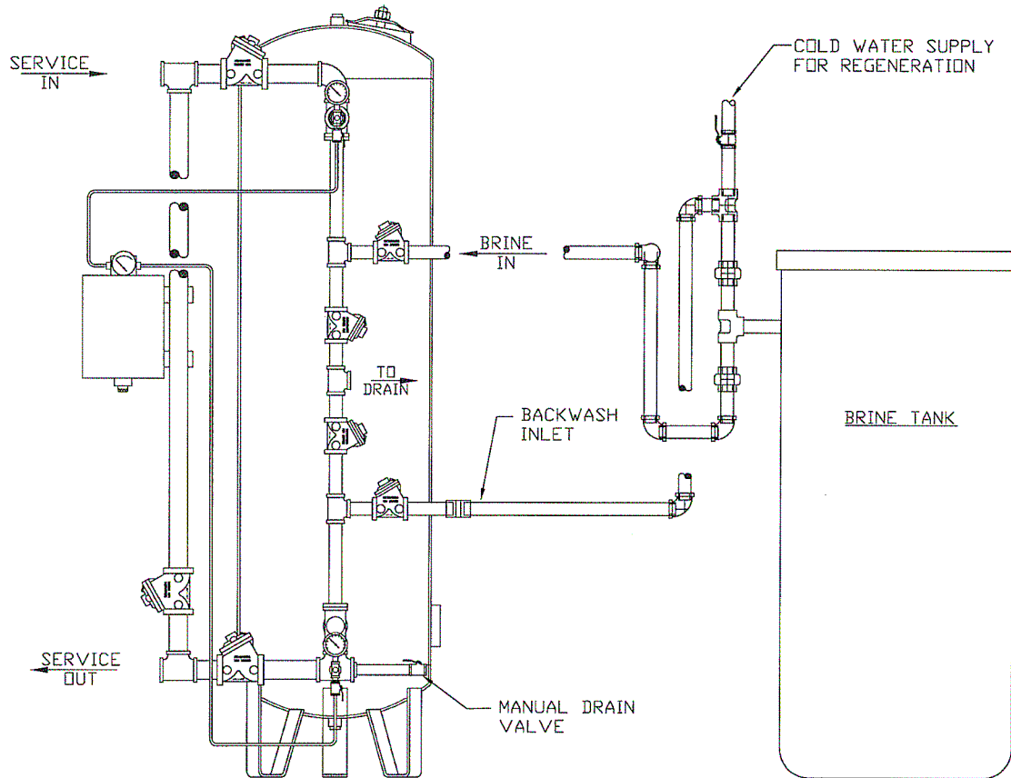
Figure 3 Drawing Of Value Engineered Condensate Polisher
