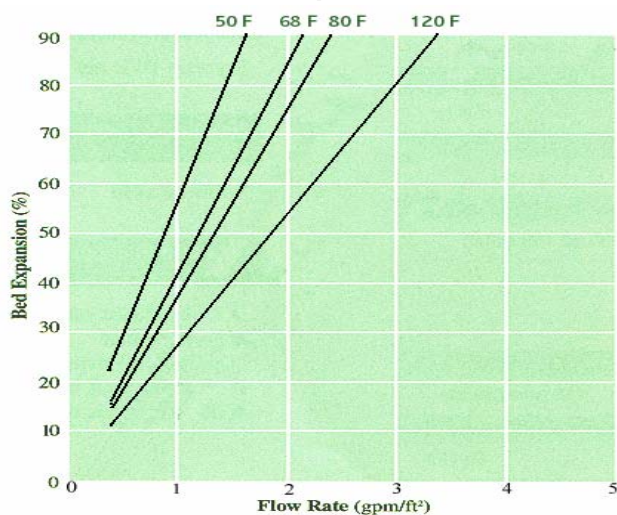
Bed Expansion Curve
