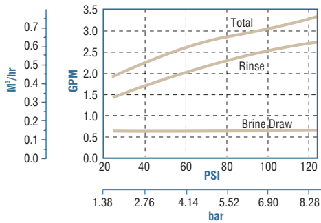
Injector # 1000443 Typical for 18-inch tank*
