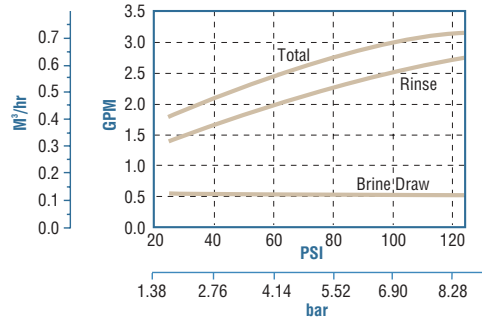
Injector # 1000442 Typical for 16-inch tank*
