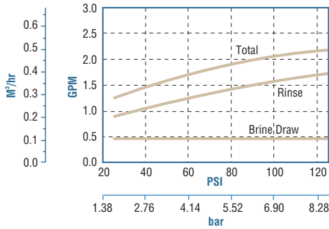
Injector # 1000441 Typical for 14-inch tank*
