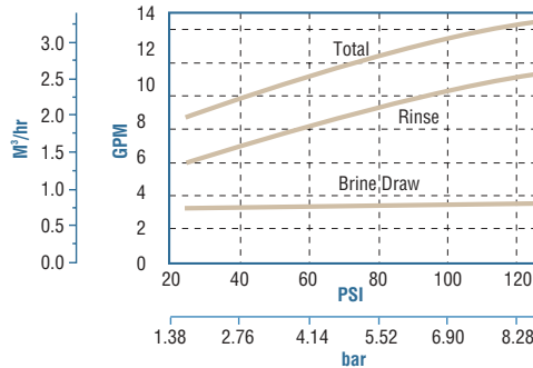
Injector # 1000447 Typical for 36-inch tank*
