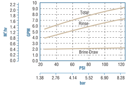
Injector # 1000446 Typical for 30-inch tank*
