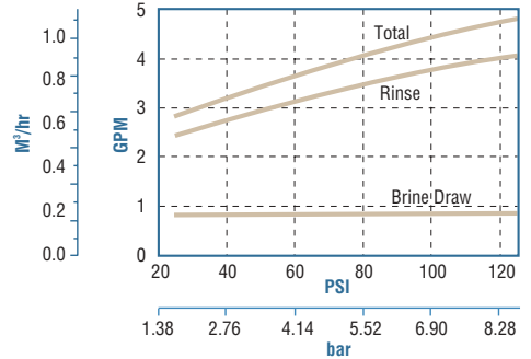
Injector # 1000444 Typical for 21-inch tank*
