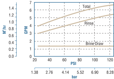
Injector # 1000445 Typical for 24-inch tank*
